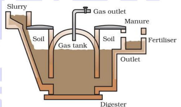
Schematic diagram of a bio-gas plant
