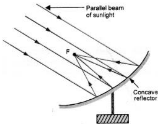
FIGURE 8. Solar Concentrator
