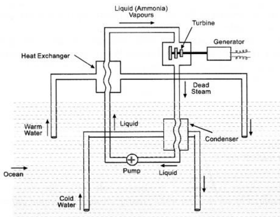
FIGURE 12 OTEC Power Plant
